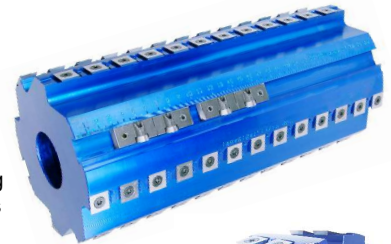
Insert Surfacing Backout Heads
